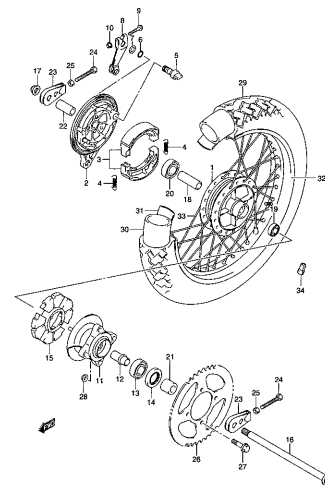
ST250XG 000_051 REAR WHEEL
