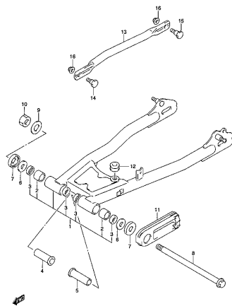
ST250XG 000_049 REAR SWINGING ARM
